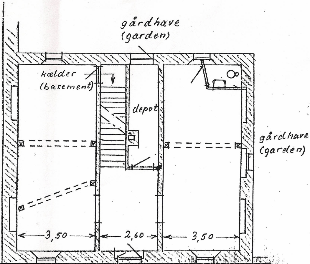
Stueetage (ground floor)
